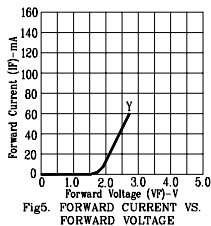
Fig5. FORWARD CURRENT VS. FORWARD VOLTAGE
