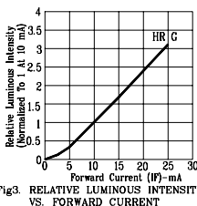
Fig3. RELATIVE LUMINOUS INTENSITY VS. FORWARD CURRENT
