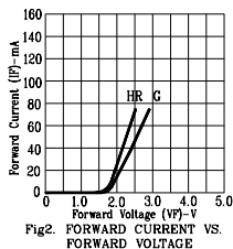
Fig2. FORWARD CURRENT VS. FORWARD VOLTAGE
