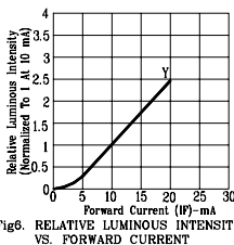
Fig6. RELATIVE LUMINOUS INTENSITY VS. FORWARD CURRENT
