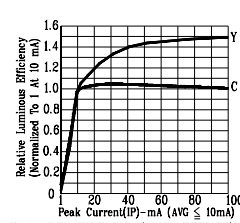
Fig7. RELATIVE LUMINOUS EFFICIENCY (LUMINOUS INTENSITY PER UNIT CURRENT) VS. PEAK CURRENT
