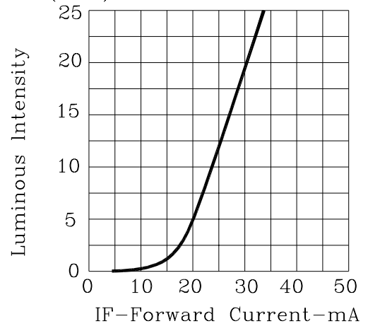
Luminous Intensity VS. Forward Current (mcd)
